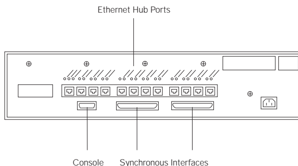
Figure 2 | 2-Port Access Node Router/Hub Connector Panel
